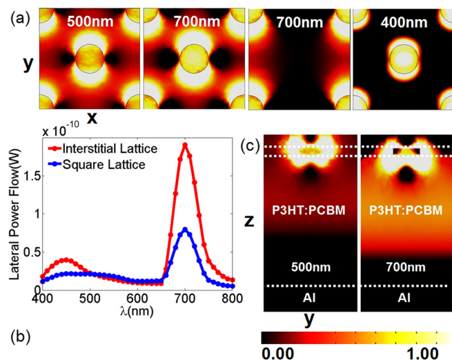
FIG. 3. (a) Top view of normalized near field profile of interstitial lattice with incident wavelength 500 nm, 700 nm, 400 nm and result of square lattice design with incident wavelength 700 nm. (b) Lateral power flow inside the active layer of OSC with interstitial lattice design ( R_A = 10 nm, R_B = 10 nm) and square lattice design ( R = 10 nm). (c) Cross section view of normalized near field profile of interstitial lattice with incident wavelength 500 nm and 700 nm. All near field profiles adopt the same normalized color bar. Normal incident light points to the negative z direction, polarized along the y direction.
