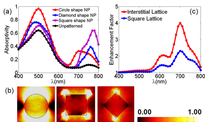
FIG. 4. (a) Absorptivity of interstitial lattice patterned OSC with NPs of different shape: circular shapes NPs, diamond shape NPs, square shape NPs, and unpatterned planar OSC. For three different patterns the size of the Ag NPs are equal to each other. (b) Normalized near field profile of different Ag NP shapes with incident wavelength \lambda = 500 nm. All near field profiles adopt the same normalized color bar. Normal incident light points to the negative z direction, polarized along the y direction. (c) Enhancement of absorptivity of interstitial lattice OSC and square lattice OSC using the Ag/MoO 3 buffer layer. All the geometric parameters are the same as Figs. 2(a) and 2(b).
