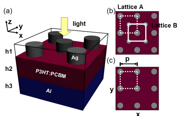
FIG. 1. (a) Schematic illustration of OSC with interstitial lattice patterned Ag nano-cylinders embedded in PEDOT:PSS. Thickness of Ag/PEDOT:PSS layer h_1 = 10 nm, P3HT:PCBM absorption layer h_2 = 100 nm, and Al layer h_3 = 100 nm. Normal incident light points to the negative z direction, polarized along the y direction. (b) Interstitial lattice pattern formed by two sets of square lattices: lattice A is denoted as dot line and lattice B is denoted as solid line. (c) Square lattice pattern. For both interstitial lattice and square lattice, the length of a unit cell is p .
