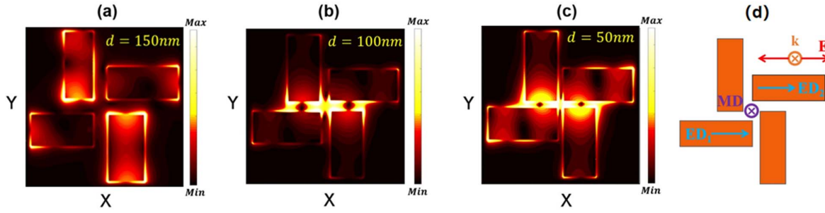
Fig. 2. Localized field distribution 2D plot at 38 THz with different spacings: (a) d = 150 nm, (b) d = 100 nm, and (c) d = 50 nm in the hybridized mode. (d) Indication of the electric dipole (ED) moment and the orthogonal magnetic dipole (MD) moment involved with the super-radiant state and the quasi BIC, respectively.
