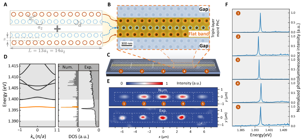
Fig. 2. Design and characterization of moiré flatband cavity. (A) Two unit cells (gray dashed rectangles) of 1D moiré PhC composed of two 1D PhCs (brown and blue circles) with slightly different lattice constants ( a_1 = 209.1 nm, a_2 = 194.1 nm). Other structural parameters: d = 133 nm, s = 95 nm, and L = 2718 nm. (B) SEM image of a fabricated triple-layer moiré PhC unit cell formed by combining two unit cells shown in (A). (C) SEM image of a moiré PhC consisting of five unit cells (white dashed rectangles). (D) Right: Comparison of calculated and experimentally measured photon DOS. The latter is obtained by spatially integrating PL spectra within a moiré PhC unit cell. The orange color indicates the flatband mode. a.u., arbitrary units. (E) Field spatial distribution of moiré flatband modes. Top: Numerical calculation accounting for the spatial resolution of the subsequent optical measurement. Bottom: PL map acquired by scanning the excitation and collection spots over the moiré PhC and recording the maximal PL intensity within 1.3939 to 1.3978 eV. The full width at half maximum (FWHM) of the excitation/collection spot is \sim 1.5 \mu m. (F) PL spectra of moiré cavity mode measured at centers of five moiré PhC unit cells marked in (C) under high-power above-barrier excitation. All experiments in this study are performed at T = 3.6 K. The Q factor of moiré cavity modes 1 to 5 are 3309, 3412, 5026, 3134, and 2602, respectively.
